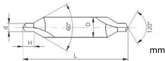
Carbide-Center Drill
